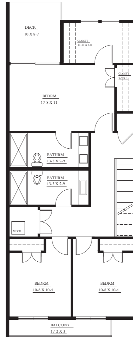
UNIT TYPE 5-INTERIOR UNIT FLOOR PLAN LEVEL TWO ALL DIMENSIONS ARE APPROXIMATE
