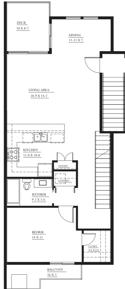
UNIT TYPE 5-INTERIOR UNIT FLOOR PLAN LEVEL ONE ALL DIMENSIONS ARE APPROXIMATE
