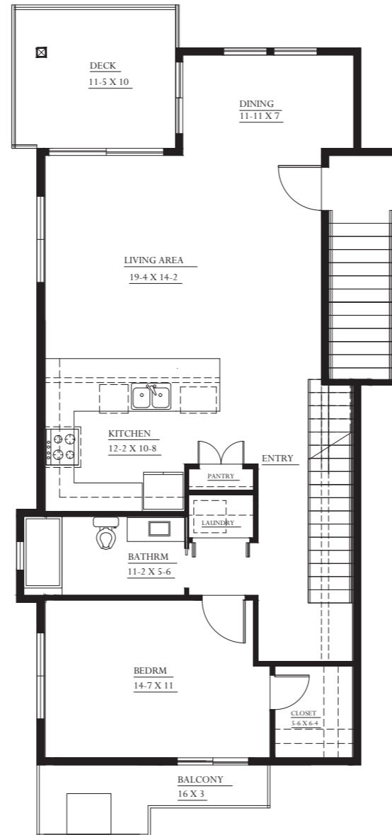
UNIT TYPE 5 -END UNIT FLOOR PLAN LEVEL ONE ALL DIMENSIONS ARE APPROXIMATE
