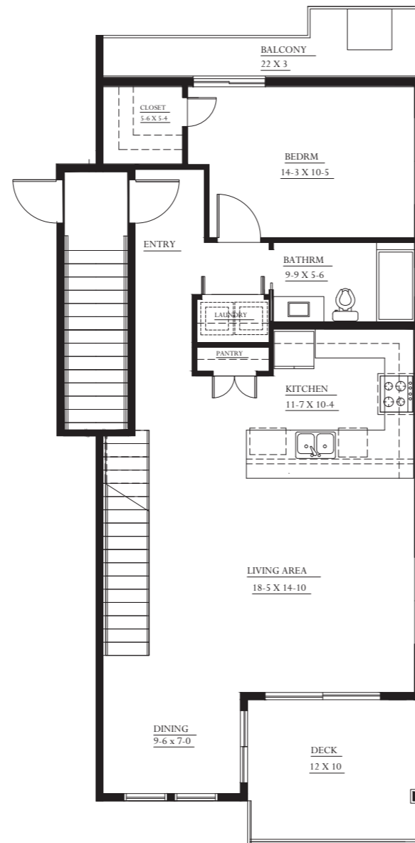
UNIT TYPE 3 - END UNIT
