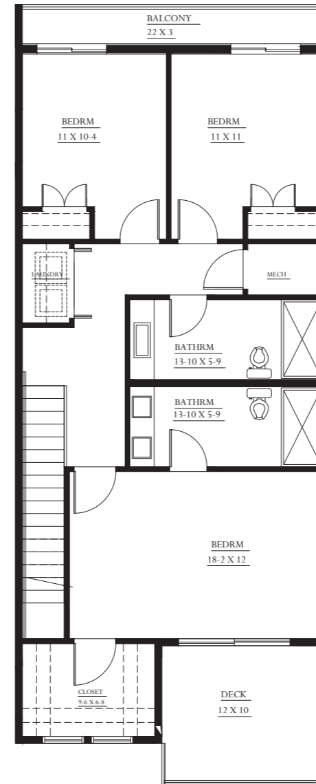
UNIT TYPE 3 - END UNIT
