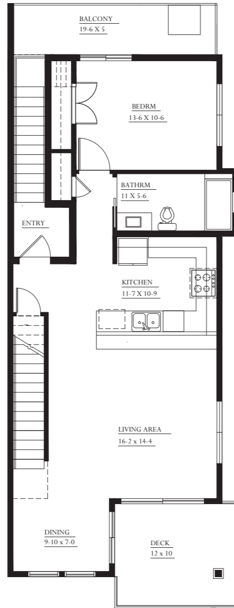
UNIT TYPE 1 - END UNIT FLOOR PLAN LEVEL ONE ALL DIMENSIONS ARE APPROXIMATE
