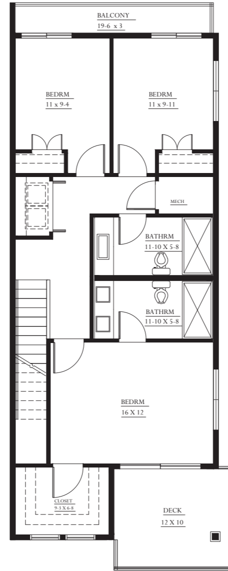
UNIT TYPE 1 - END UNIT FLOOR PLAN LEVEL TWO ALL DIMENSIONS ARE APPROXIMATE
